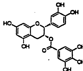
EPICATECHIN GALLATE
